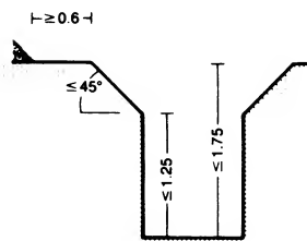
8 Excavation with banked edges
